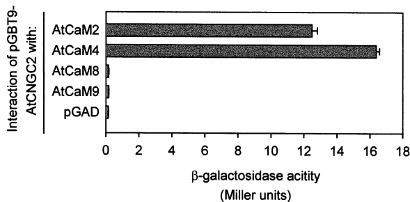
Fig. 5. Quantitative analysis of interactions of AtCNGC1 (a) and AtCNGC2 (b) C-terminal peptides with AtCaM2, AtCaM4, AtCaM8 and AtCaM9 in yeast. The graphs indicate the \beta -galactosidase reporter activity in yeast cells corresponding to the combinations of transformed constructs. For each combination at least six assays were performed. Error bars represent S.E.M.
