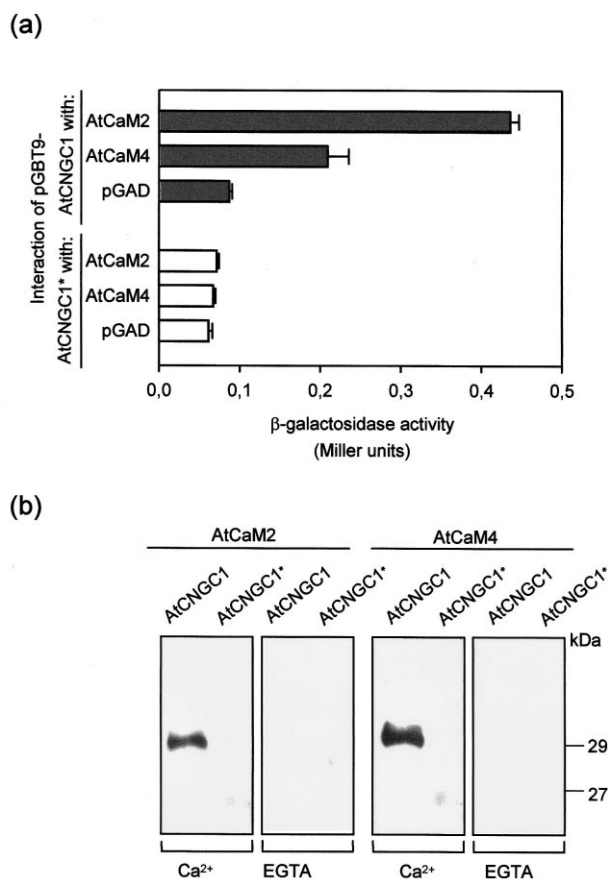
Fig. 2. Deletion of the calmodulin binding site of AtCNGC1 abolished binding of calmodulin. a: Quantitative two-hybrid analysis of interaction of AtCNGC1 C-terminal peptides with AtCaM2 and AtCaM4 in yeast. AtCNGC1* corresponds to the AtCNGC1 C-terminal peptide with the calmodulin binding site deleted. The graphs indicate the \beta -galactosidase reporter activity in yeast cells corresponding to the combinations of transformed constructs. For each combination at least six assays were performed. Error bars represent S.E.M. b: Calmodulin overlay analysis with Strep -tagged calmodulins and the purified C-terminal peptides of AtCNGC1 and AtCNGC1*. The calculated M_r s of the AtCNGC1 and AtCNGC1* C-terminal peptides are 29 and 26.8 kDa, respectively. Proteins (0.5 \mu\text{g} ) were separated by SDS-PAGE, subjected to Western blot and incubated with Strep -tagged calmodulin in the presence of either 5 mM \text{CaCl}_2 or 5 mM EGTA.
